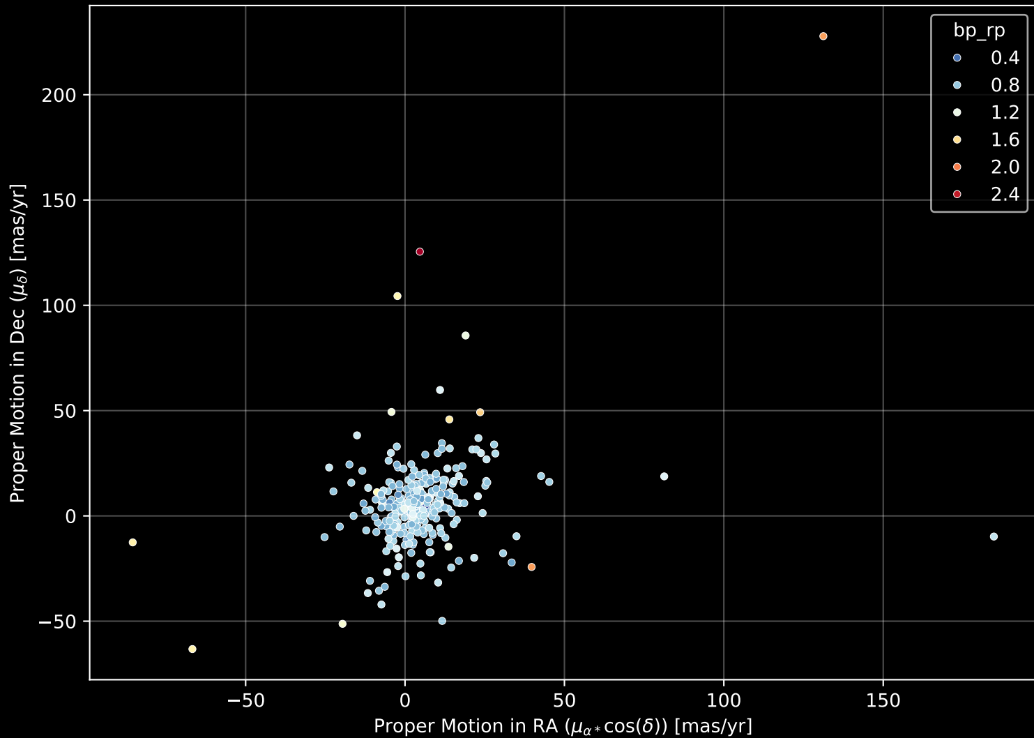
GALAH DR4 Field: [451] Proper Motion Diagram (n= 302)
