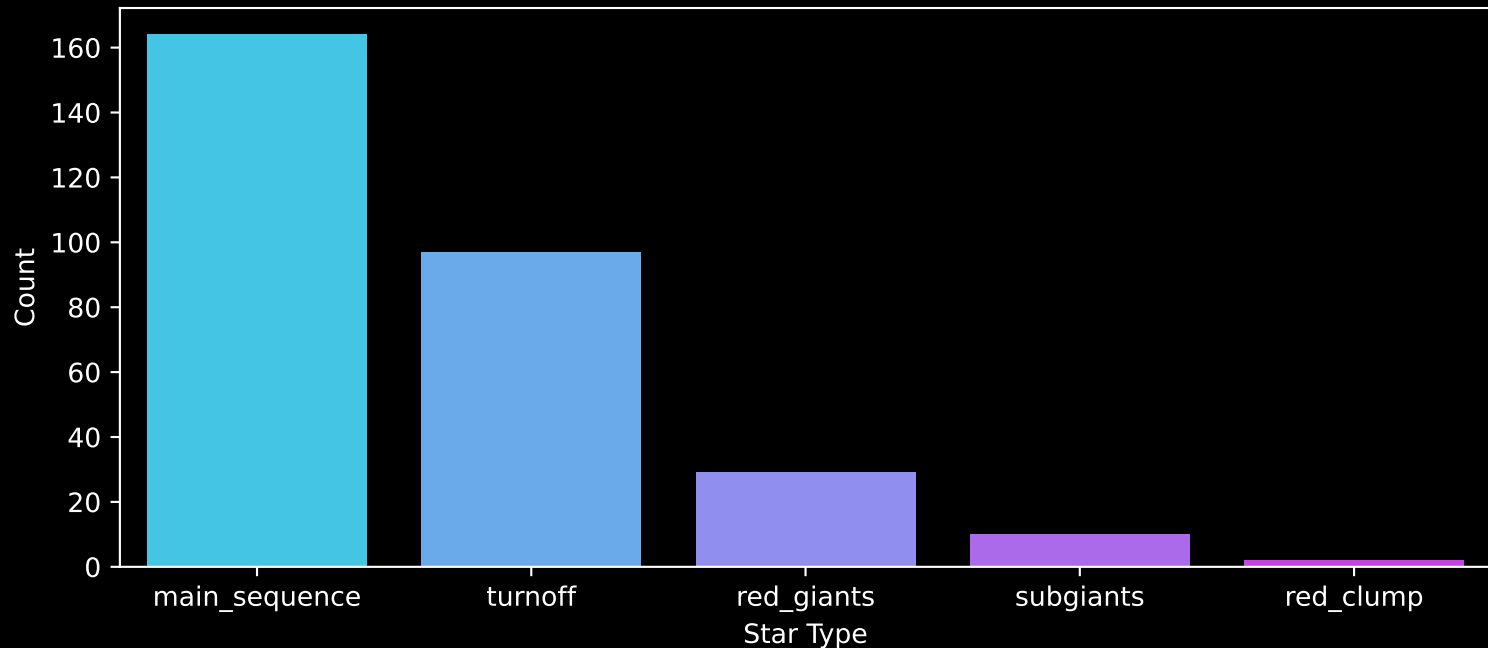
GALAH DR4 Field: [451] Count plot of Star Type
