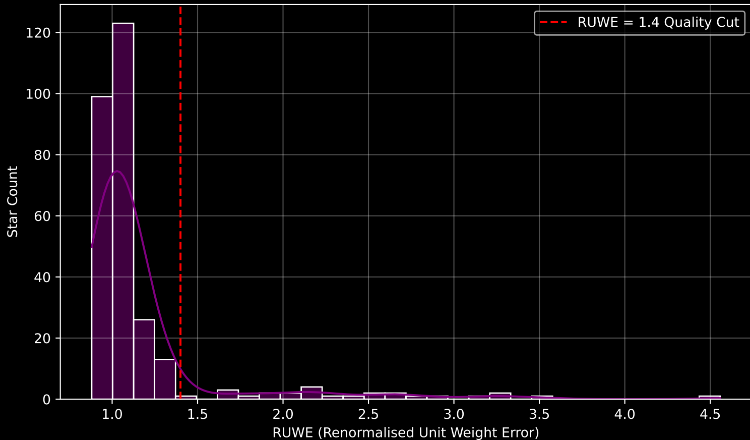
GALAH DR4 Field [451] RUWE Distribution (n= 287)
